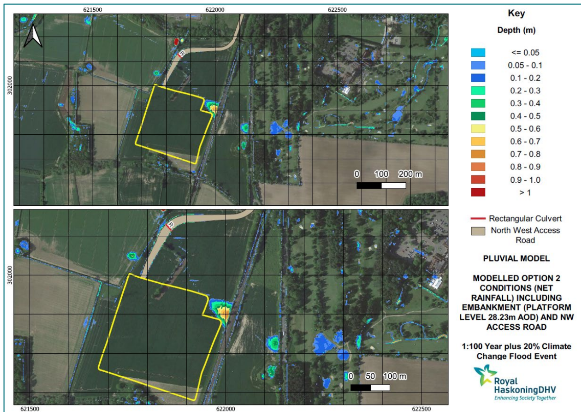
Figure 9-219-21: 1 in 100 year plus 20% for climate change with OnSS platform level set at 28.23m AOD and NW access road
