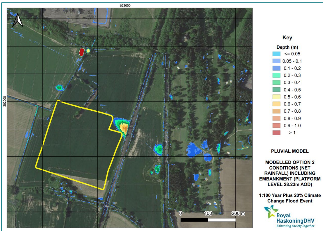
Figure 9-189-18: 1 in 100 year plus 20% for climate change with OnSS platform level set at 28.23m AOD
