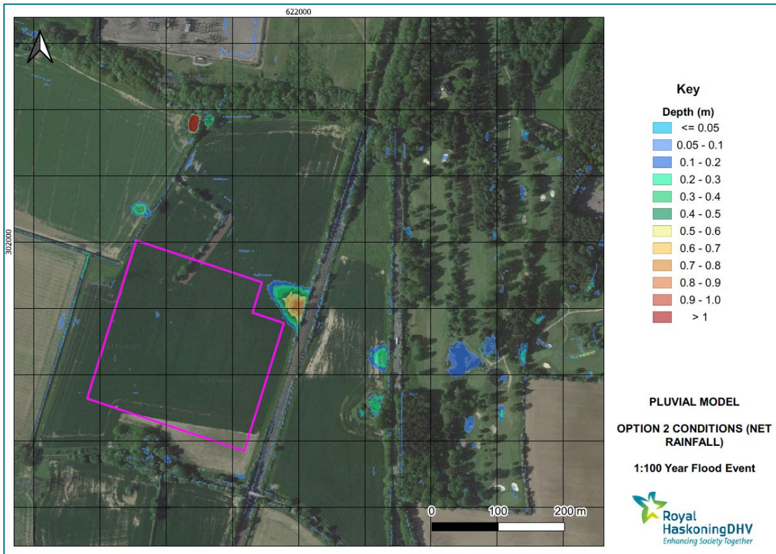
Figure 9-89-8: 1 in 100 year extent in comparison with Option 2 layout using net rainfall hyetograph
