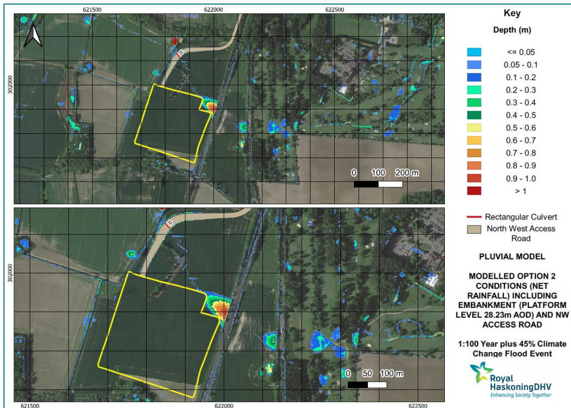
Figure 9-239-23: 1 in 100 year plus 45% for climate change with OnSS platform level set at 28.23m AOD and NW access road
