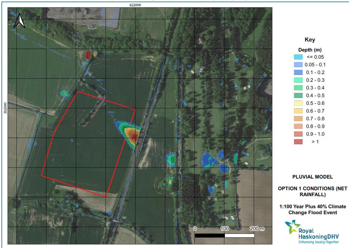
Figure 9-49-4: 1 in 100 year plus 40% for climate change extent in comparison with Option 1 layout using net rainfall hyetograph
