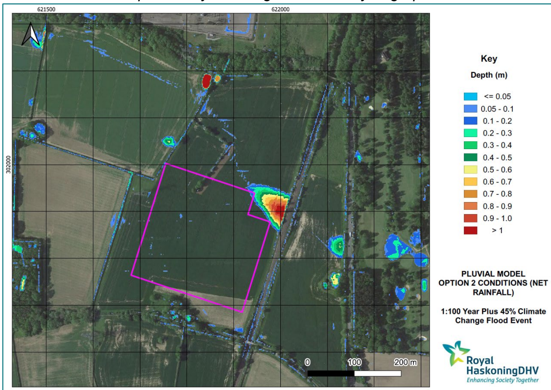
Figure 9-119-11: 1 in 100 year plus 45% for climate change extent in comparison with Option 2 layout using net rainfall hyetograph
