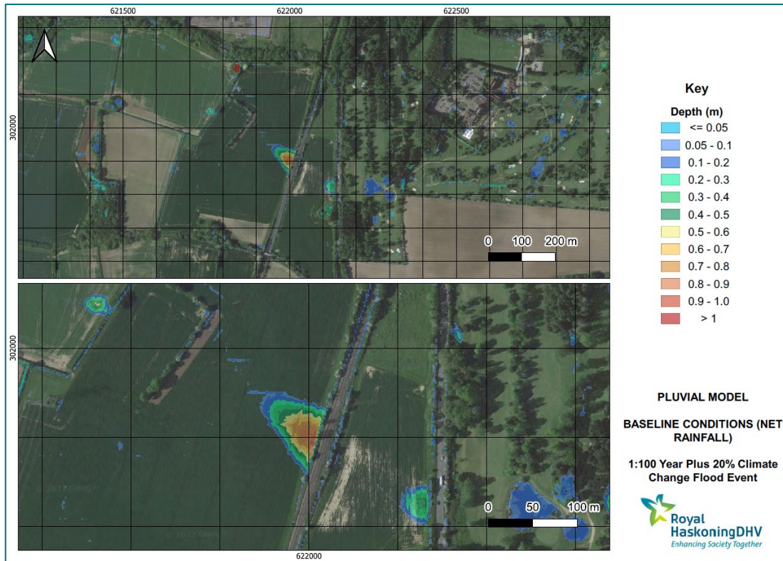
Figure 8-88-8: 1 in 100 year plus 20% for climate change Baseline (existing) using net rainfall hyetograph
