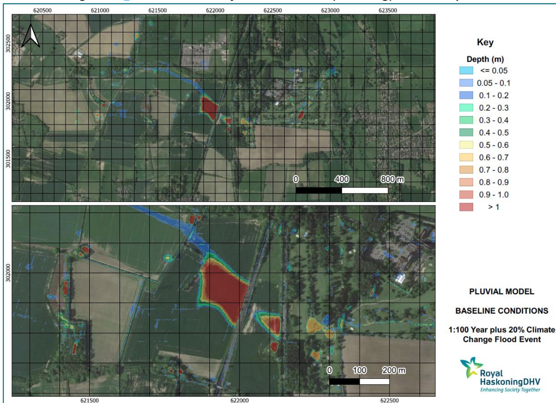
Figure 8-28-2: 1 in 100 year Baseline (existing) flood depth
