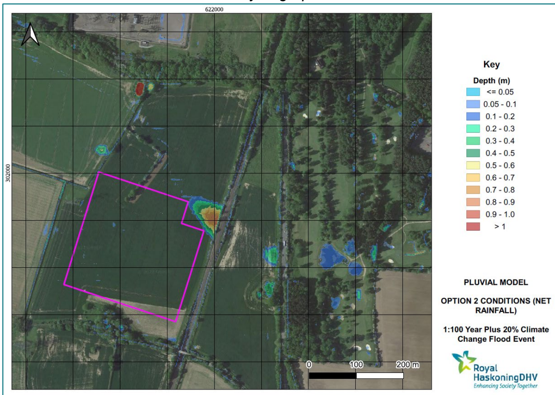
Figure 9-99-9: 1 in 100 year plus 20% for climate change extent in comparison with Option 2 layout using net rainfall hyetograph
