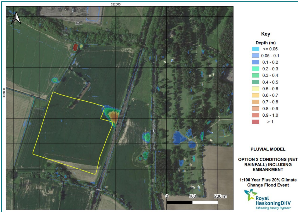
Figure 9-159-15: 1 in 100 year plus 20% for climate change extent in comparison with Option 2 embankments layout
