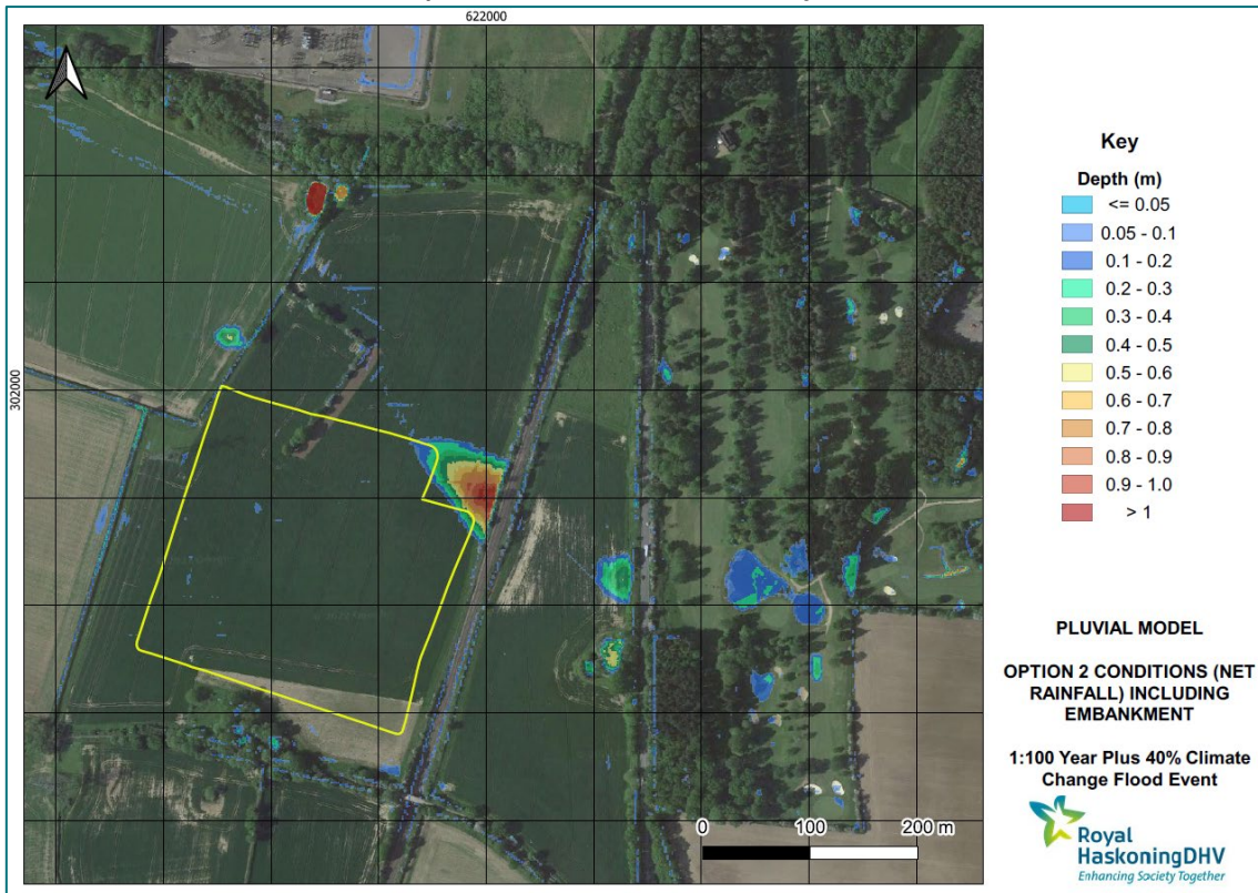
Figure 9-169-16: 1 in 100 year plus 40% for climate change extent in comparison with Option 2 embankments layout
