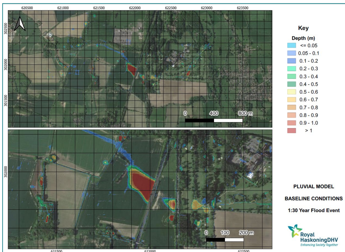
Figure 8-18-1: 1 in 30 year Baseline (existing) flood depth
