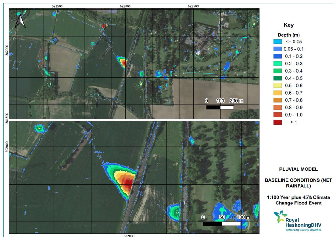
Figure 8-108-10: 1 in 100 year plus 45% for climate change Baseline (existing) using net rainfall hyetograph
