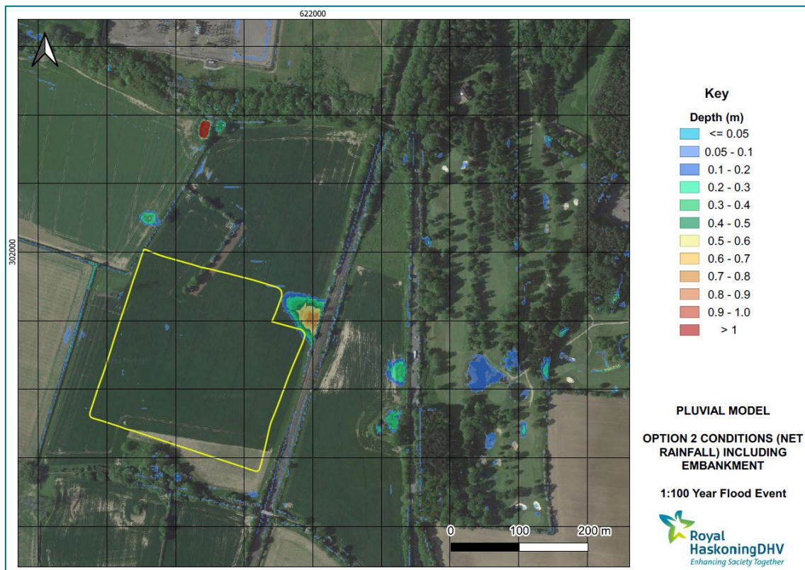
Figure 9-149-14: 1 in 100 year extent in comparison with Option 2 with embankments layout
