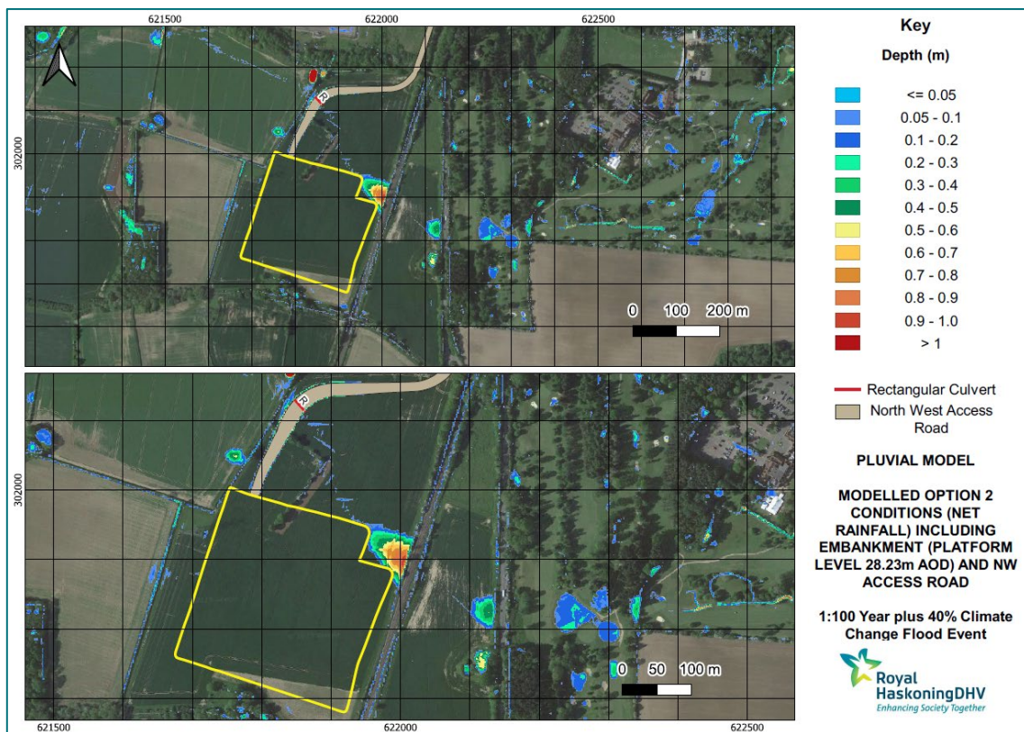
Figure 9-229-22: 1 in 100 year plus 40% for climate change with OnSS platform level set at 28.23m AOD and NW access road
