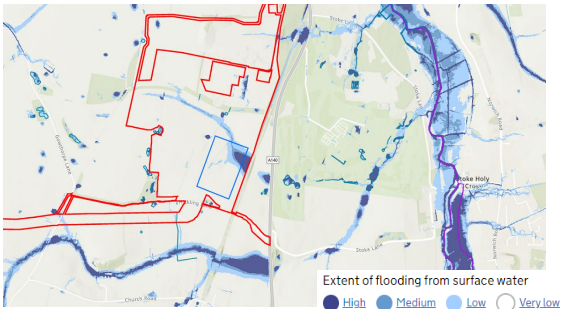
Figure 2-12-4: Extract of Environment Agency surface water flood risk mapping in comparison with the proposed OnSS platform (at the time of the initial review)
