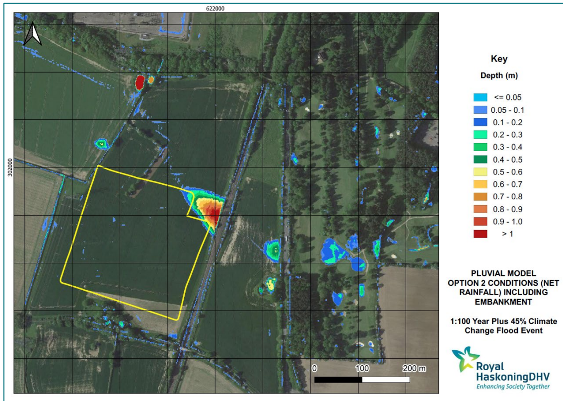
Figure 9-179-17: 1 in 100 year plus 45% for climate change extent in comparison with Option 2 embankments layout
