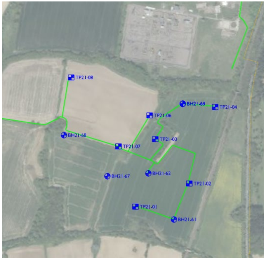
Figure 3-23-2: September 2021 exploratory hole locations
